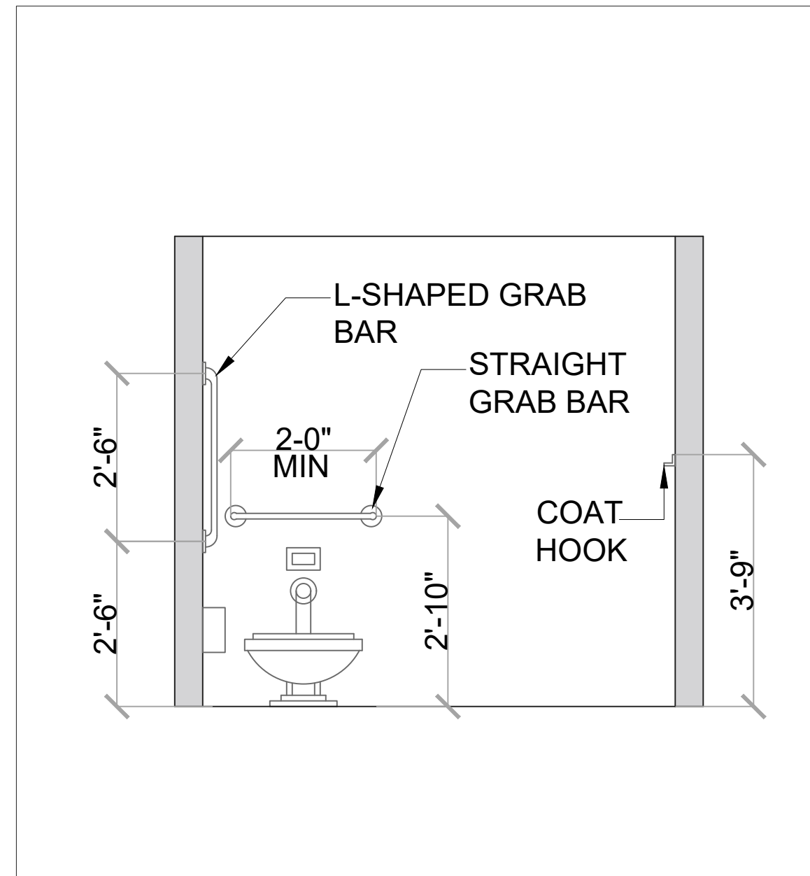
ELEVATION AMBULATORY 1
