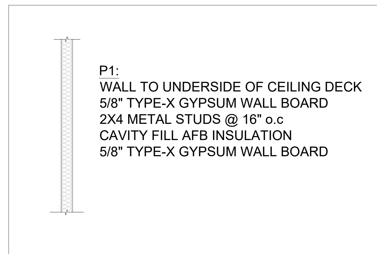
PARTITION 1 DETAILS FOR NEW WALLS
