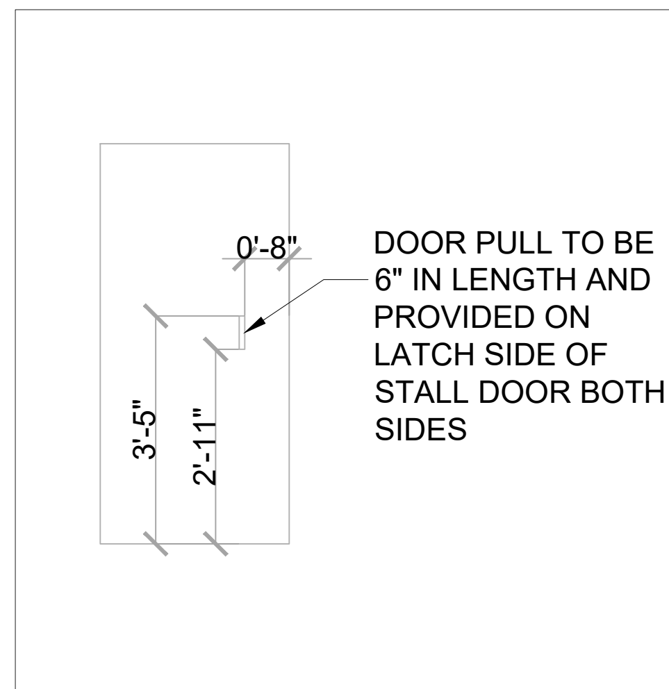
DETAIL 1
