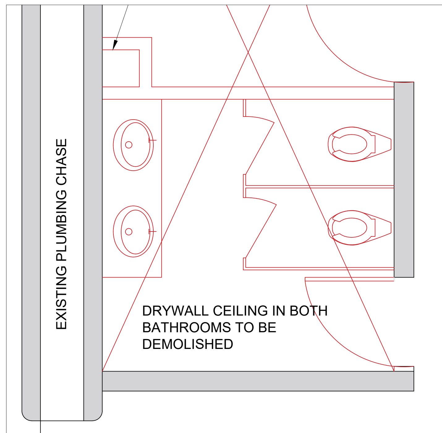
C2125 WOMENS DEMOLITION PLAN
