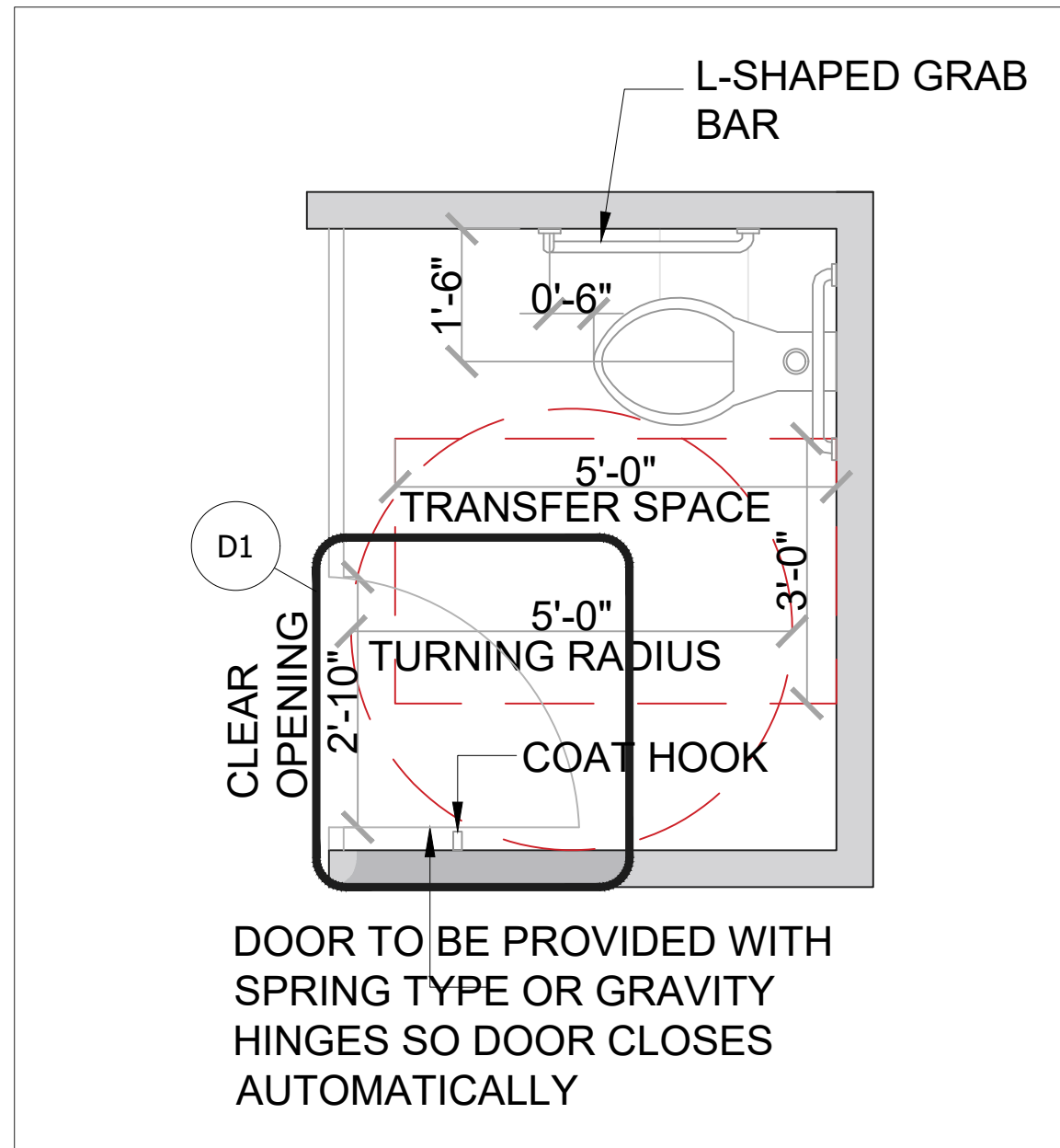
LAYOUT
