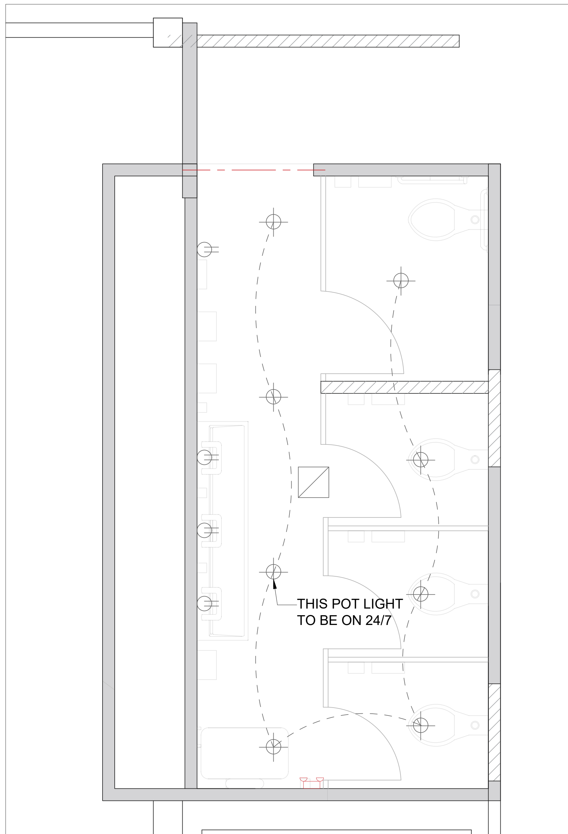
NEW PROPOSED RESTROOM REFLECTED CEILING PLAN
