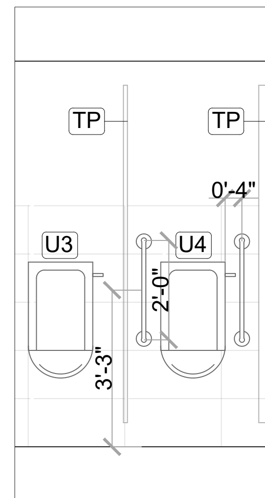
ELEVATION AMBULATORY URINAL
