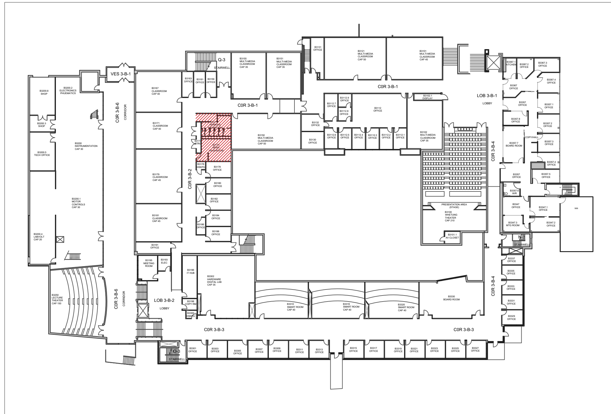
B-WING RESTROOM LOCATION
