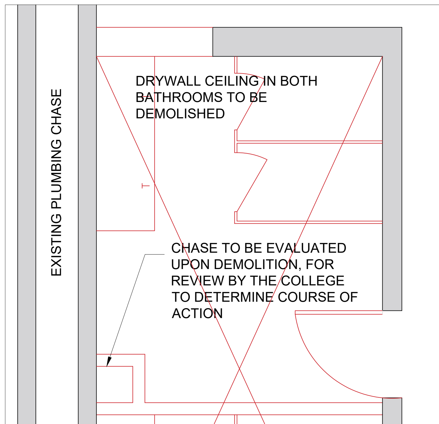
C2126 MENS DEMOLITION PLAN
