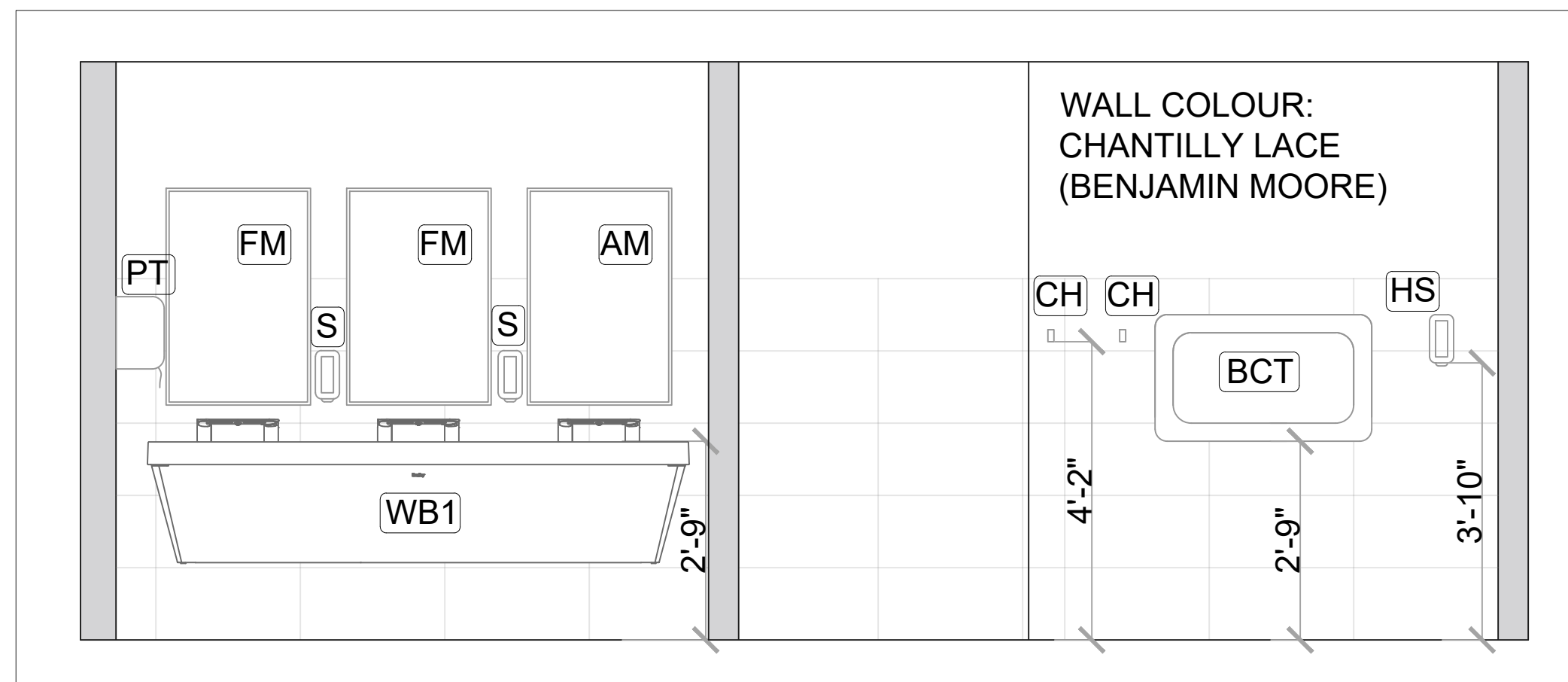
B3174 ELEVATION 3.1
