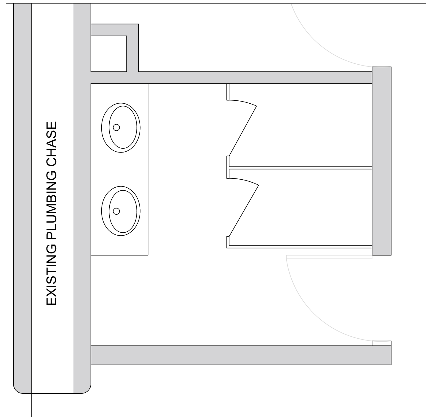
C2125 WOMENS RESTROOM LAYOUT
