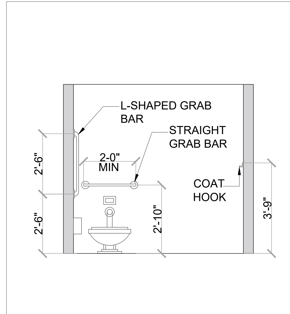
ELEVATION BF1
