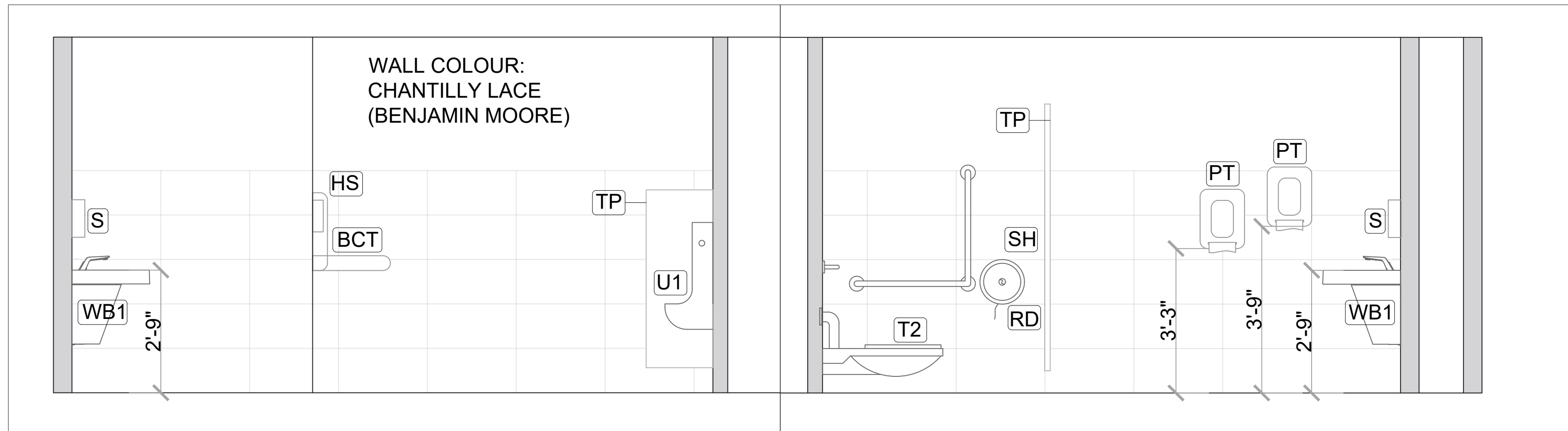
B3174 ELEVATION 1.1
